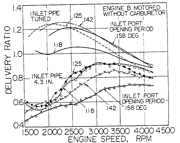
Fig. 20 - Effect of inlet port opening period
