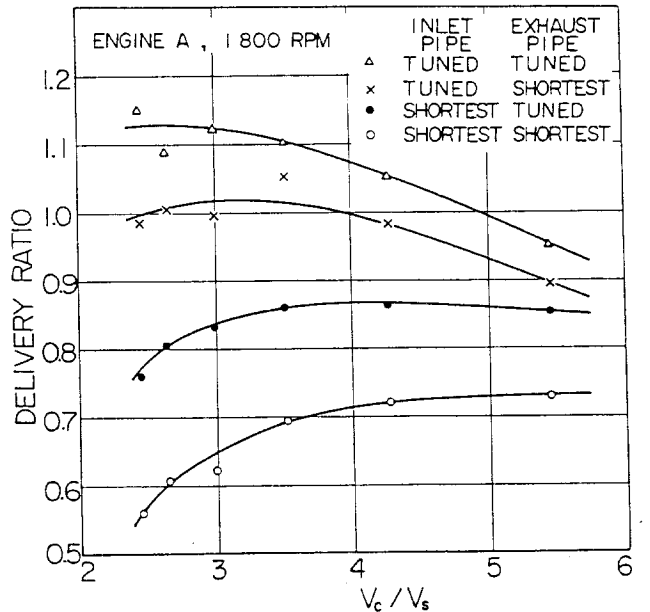
Fig. 8 - Effect of crankcase clearance volume V_c
