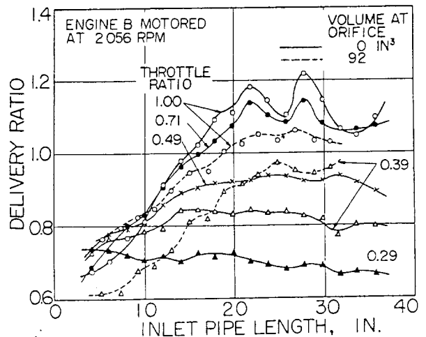
Fig. 26 - Effect of orifice fixed to external end of inlet pipe
